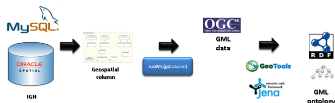
Figure 1: Transformation of the geospatial information into RDF
